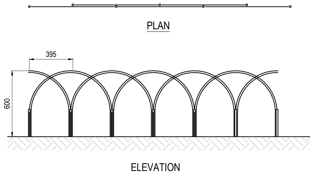
STEEL HOOP BARRIER TYPICAL SETOUT
