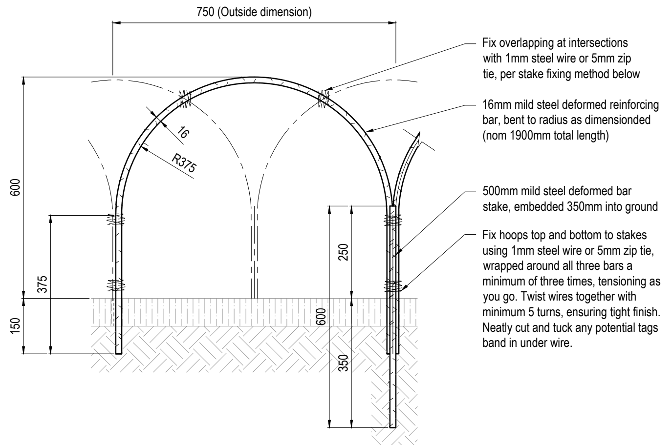
STEEL HOOP BARRIER TYPICAL SETOUT
