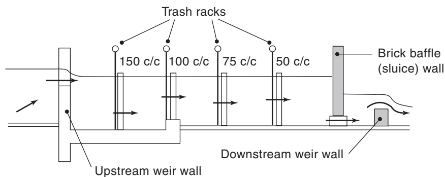
Figure 7.15 Hydraulically operated trash racks (after Townshend 1996).
