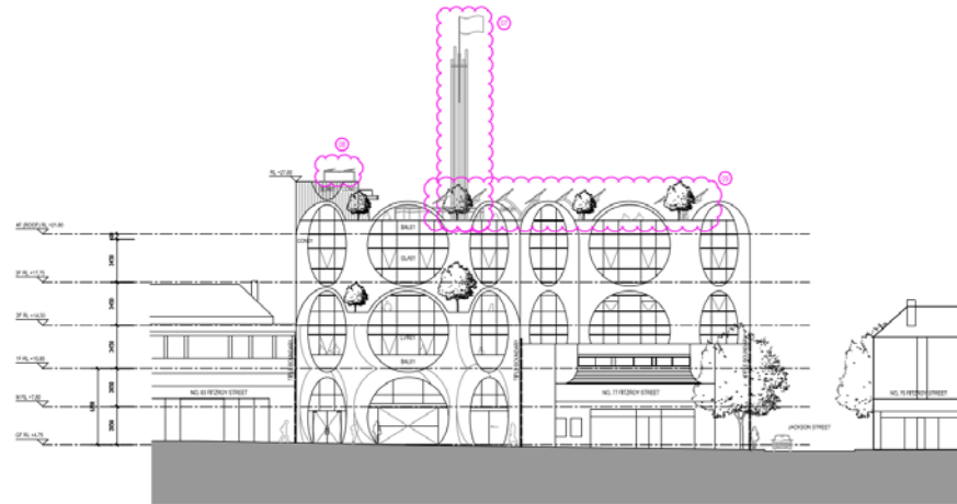
After: Fitzroy Street (front) Elevation
