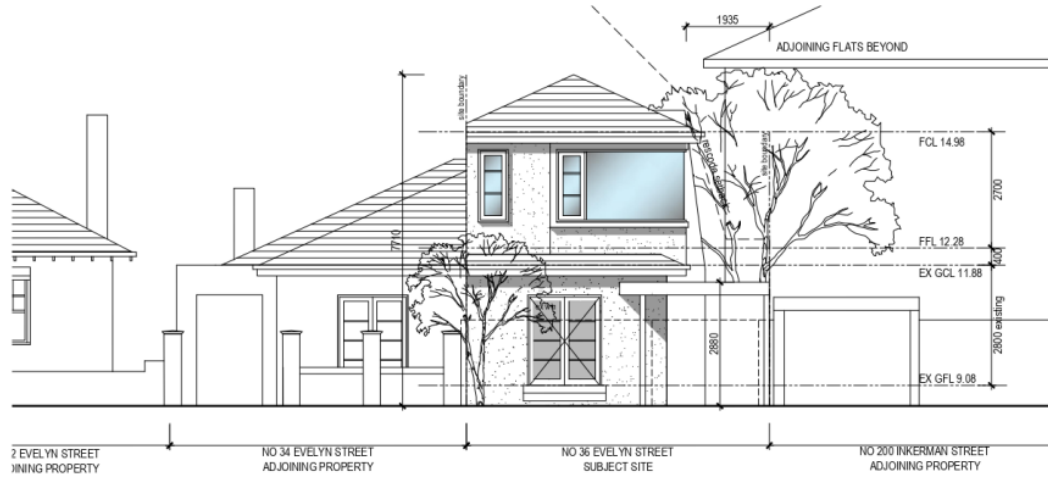
west elevation
