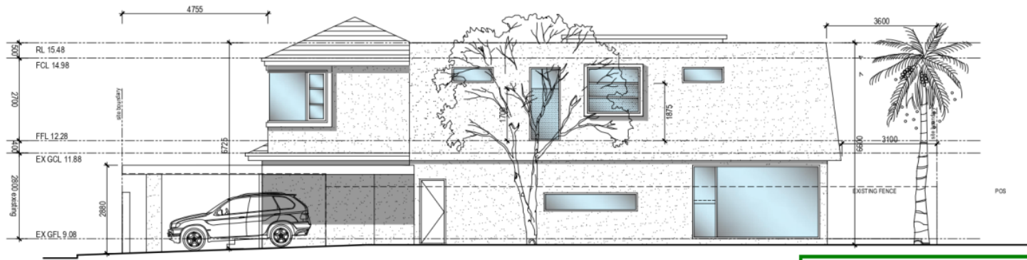
south elevation
