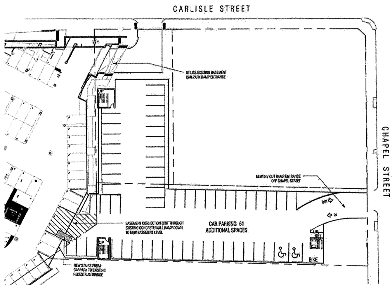
PROPOSED BASEMENT PLAN
