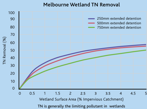
Figure 1 Sizing curve for wetlands in Melbourne
