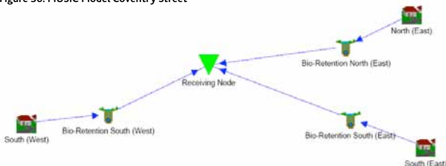
Figure 36. MUSIC Model Coventry Street
