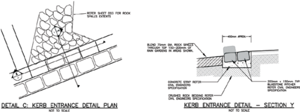
Figure 35. Kerb entrance and section detail
