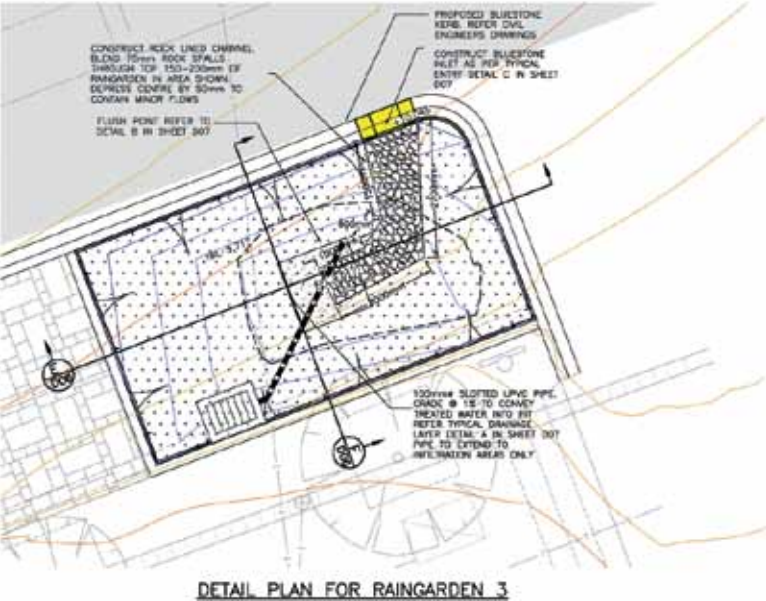
Figure 34. Plan view of raingarden 3 showing drainage and surface details
