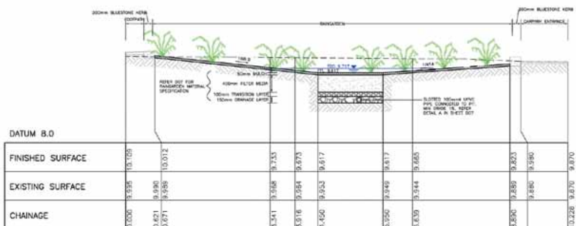
Figure 33. Section detail of Raingarden 3
