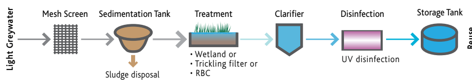
Figure 12. Typical treatment train for a greywater reuse system
