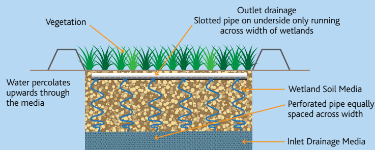
Figure 1 Typical subsurface flow wetland – section drawing
